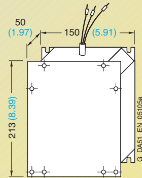
Choke for upright mounting 6SE6400-3CC02-6BB3
