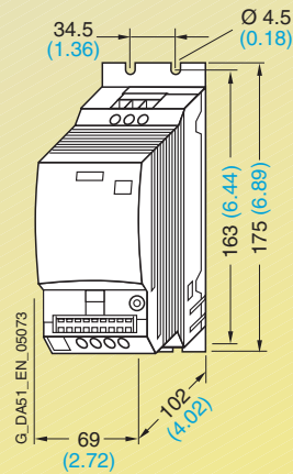
Inverter with flat plate heatsink 6SE6410-2 . B13-7AB0 6SE6410-2 . B17-5BB0
