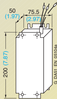
Footprint chokes 6SE6400-3CC00-4AB3 6SE6400-3CC01-0AB3
